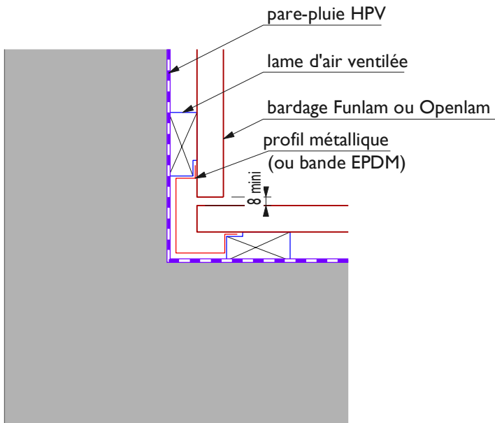
joint creux
